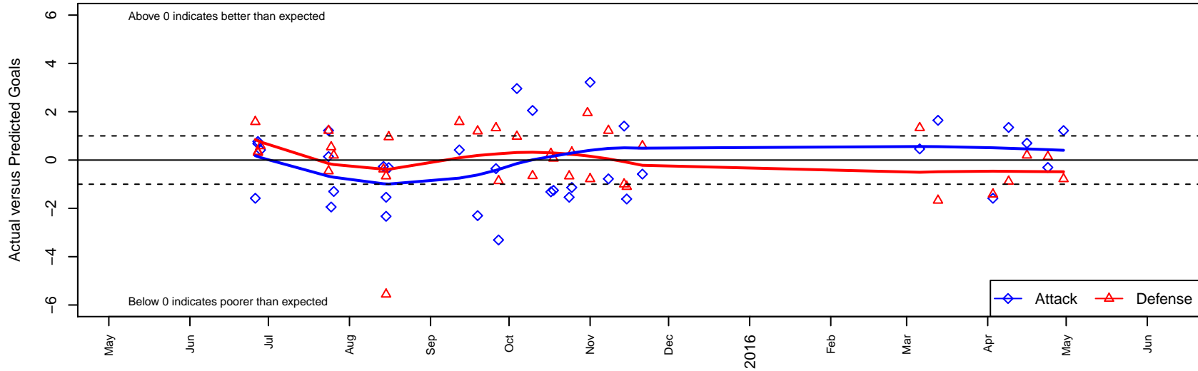
Capital FC Timbers Black B02 Dots are actual minus expected GF (blue circles) and GA (red triangles). Blue line is smoothed change in attack strength. Red is smoothed change in defense strength.
